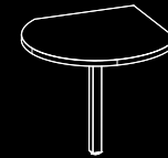
Teardrop table, 60x60 cm or Ø 60 mm metal leg on adjustable foot Melamine top (T 40 mm) Code 15492 Sandblasted glass top (T 10 mm) Code 15493
