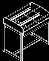
Double melamine comic and album browser, free-standing H 81cm H 51 cm W 60 cm Code 21466 Code 21467 W 90 cm Code 21468 Code 21469 W 120 cm Code 21470 Code 21471
