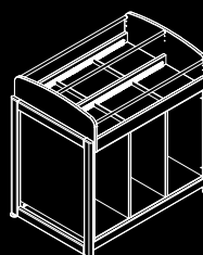
Double melamine comic and album browser with compartments, free-standing H 81cm W 60 cm Code 21472 W 90 cm Code 21473 W 120 cm Code 21474
